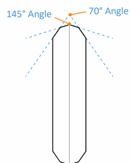
Double Sharpened Grind
